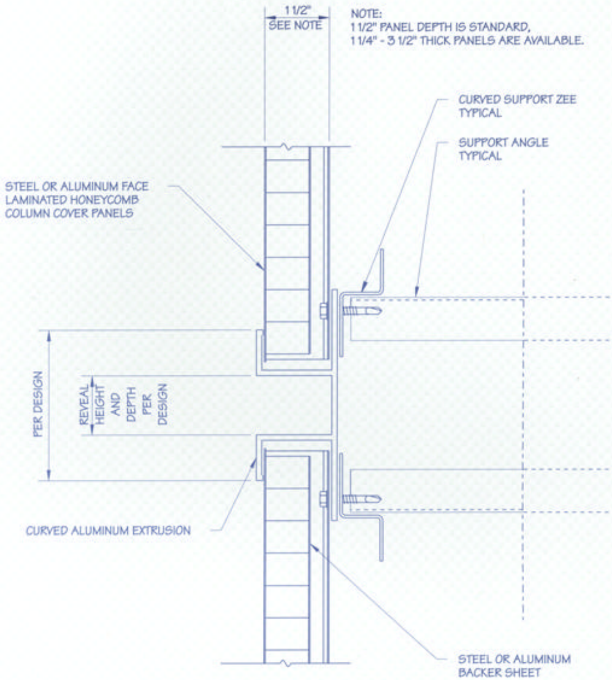
SECTION "B2-B2"
