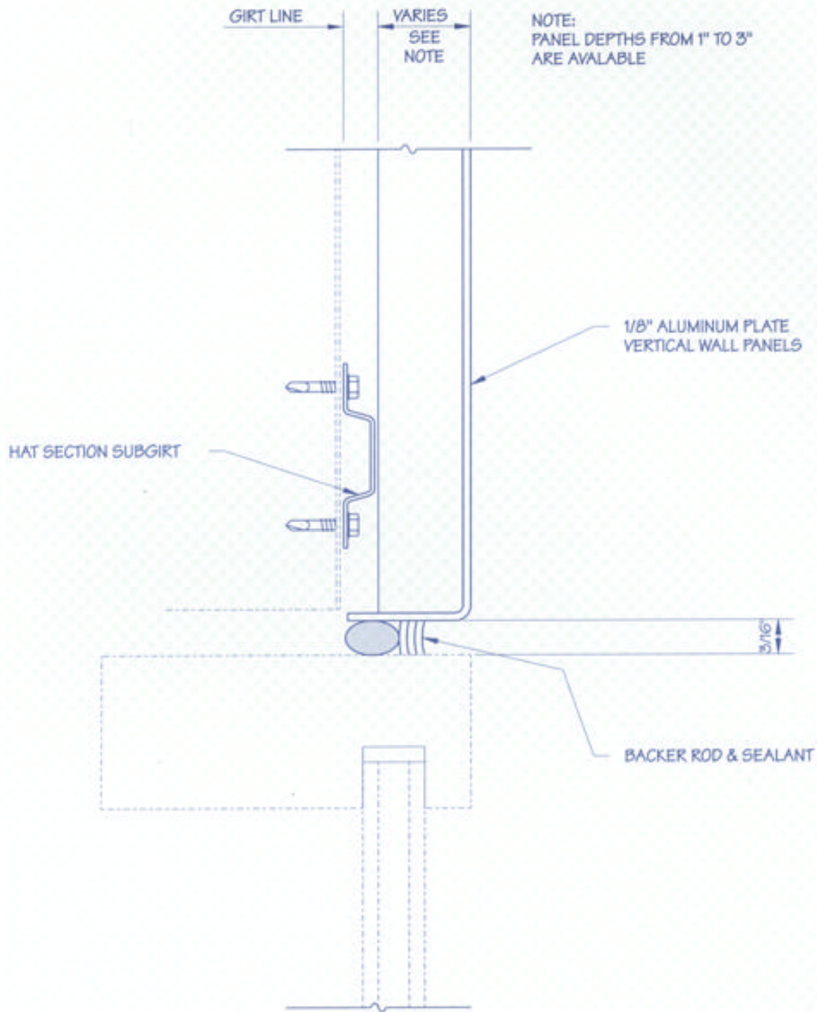
TYPICAL PANEL WINDOW, DOOR & LOUVER HEAD
