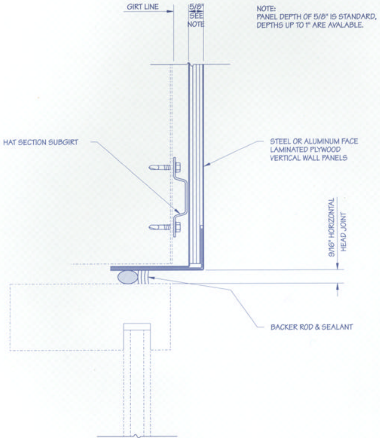
TYPICAL PANEL WINDOW, DOOR & LOUVER HEAD TYPICAL PANEL WINDOW, DOOR & LOUVER JAMB (SIMILAR)
