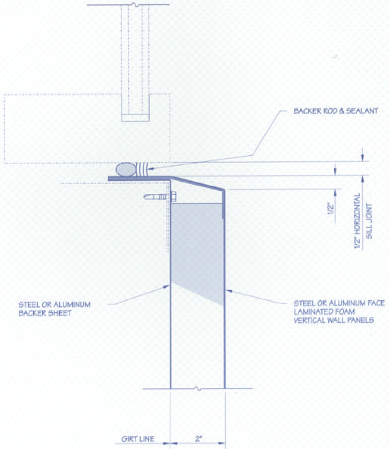
TYPICAL PANEL WINDOW & LOUVER SILL
