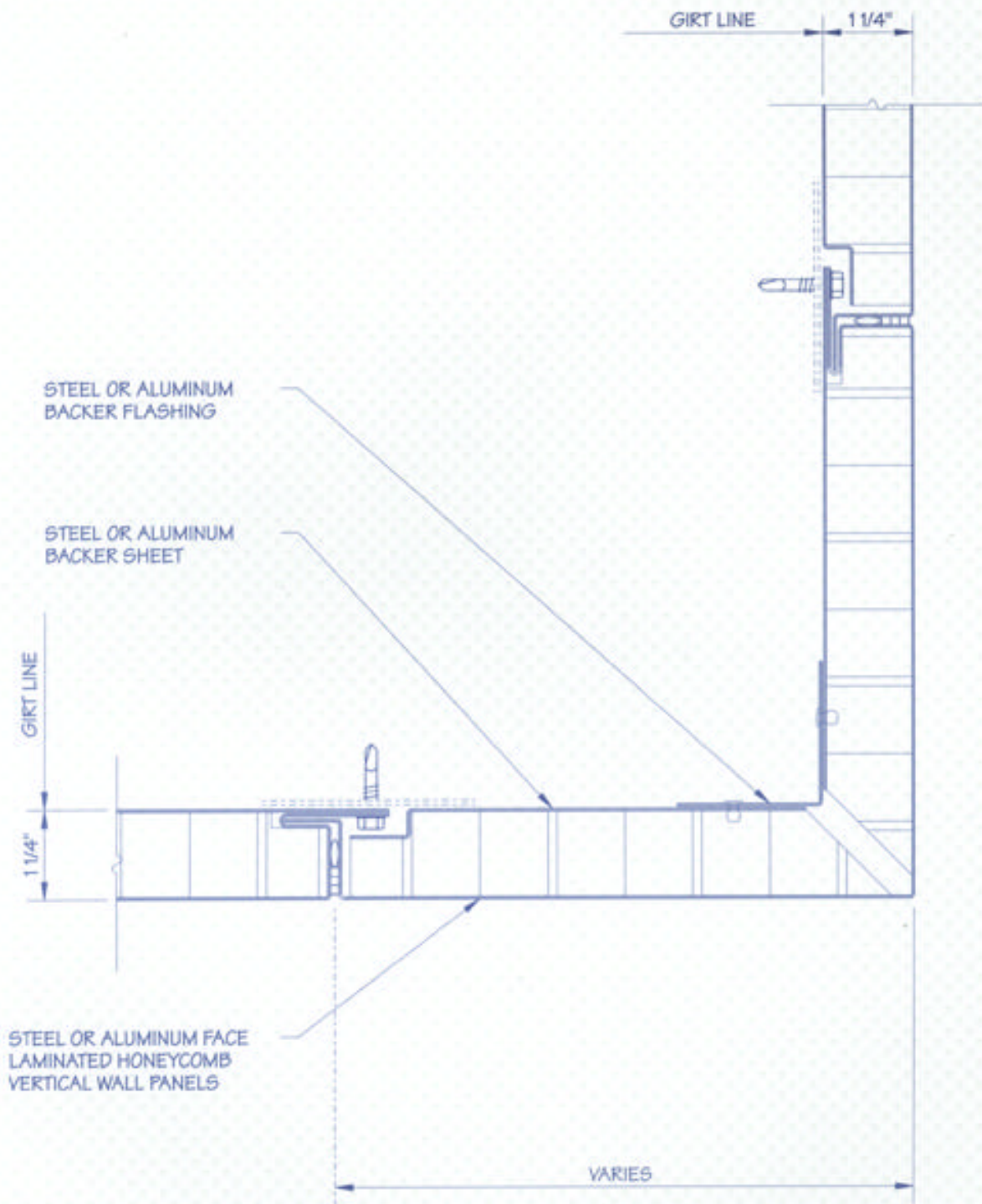
TYPICAL PANEL TRIMLESS OUTSIDE CORNER
