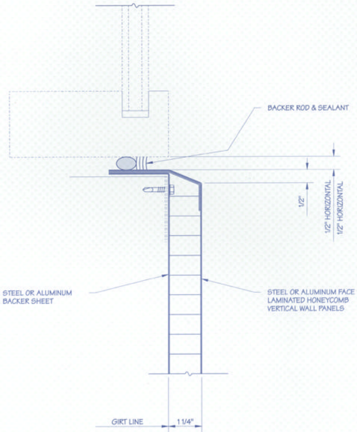
TYPICAL PANEL WINDOW & LOUVER SILL
