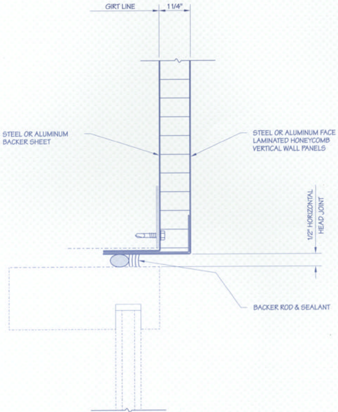
TYPICAL PANEL WINDOW, DOOR & LOUVER HEAD TYPICAL PANEL WINDOW, DOOR & LOUVER JAMB (SIMILAR)
